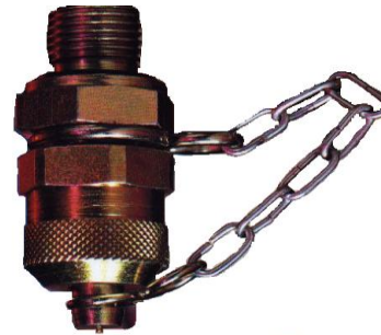
MINITEST COUPLING SIZE:- M16-2.0 x 1/4" BSP
